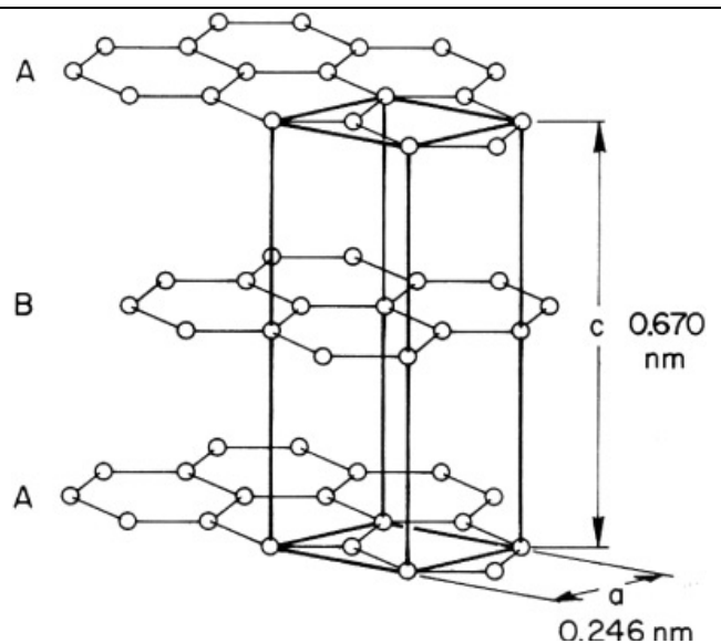
Figure 6: Crystal structure of Graphite
