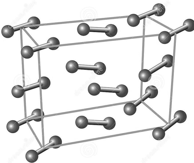
Figure 5: Crystal Structure of Iodine
