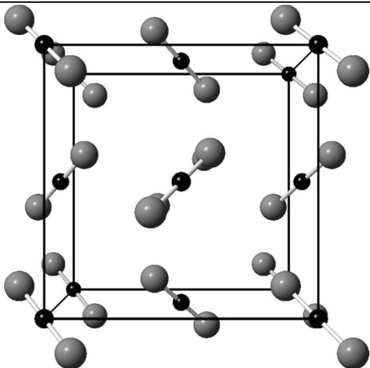
Figure 7: Crystal structure of solid CO 2
