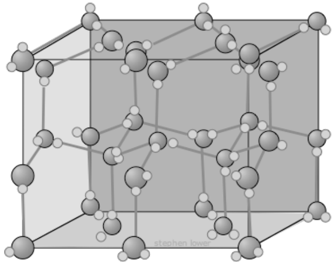
Figure 4: Crystal structure of Ice
