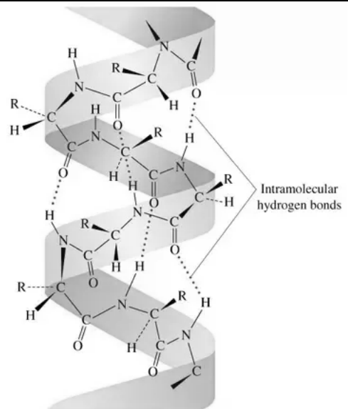
Figure 10 : Hydrogen bonds in Proteins
