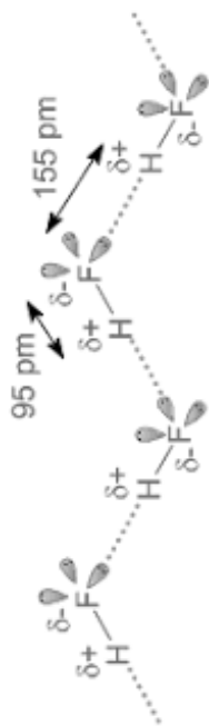
Figure 11 : Hydrogen bonds in HF
