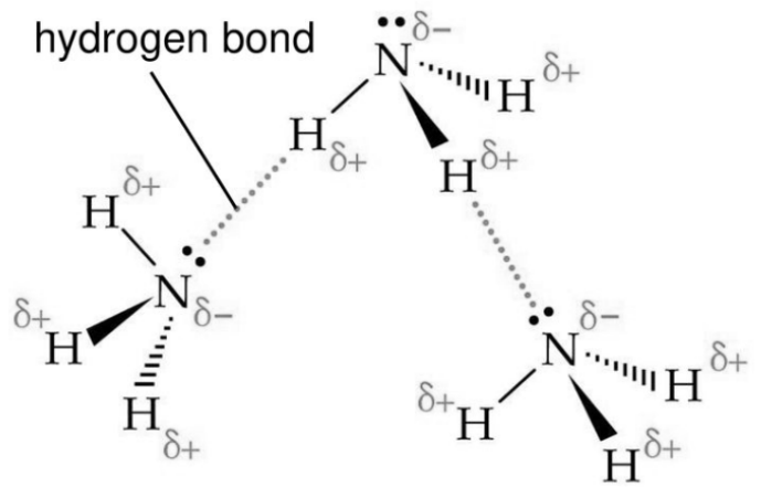
Figure 8: Hydrogen bonds in liquid NH 3
